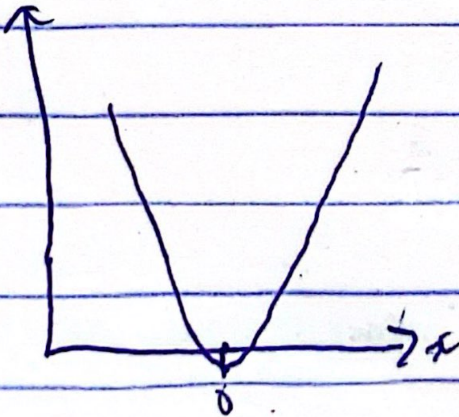
fig 2. parabolic potential energy curve.
