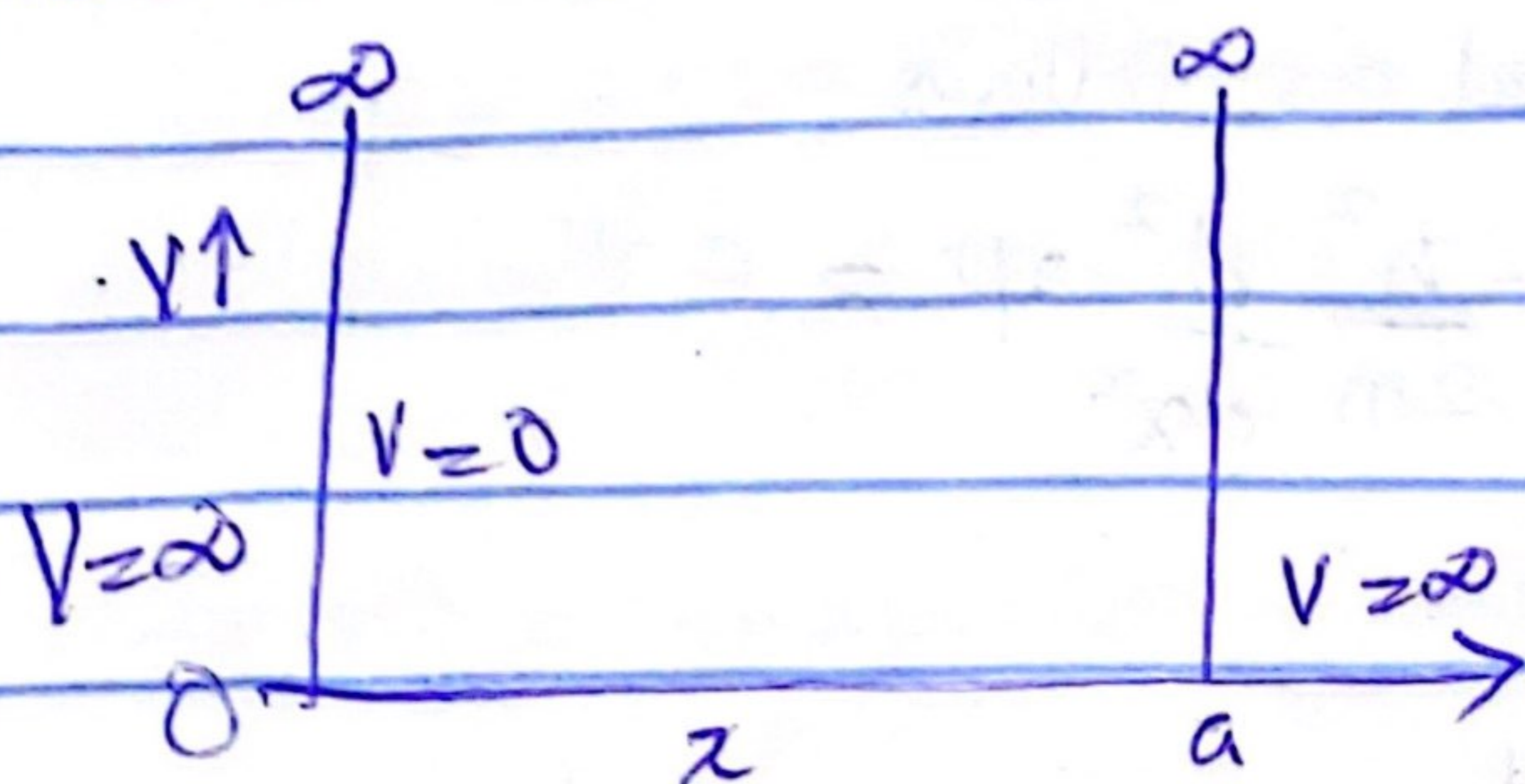
fig 5: potential energy for particle in a box
