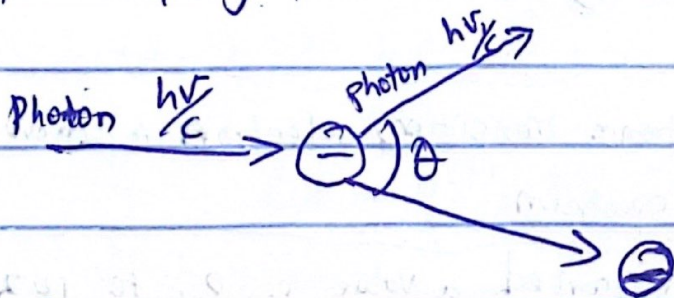
Fig 4: The Compton effect.
