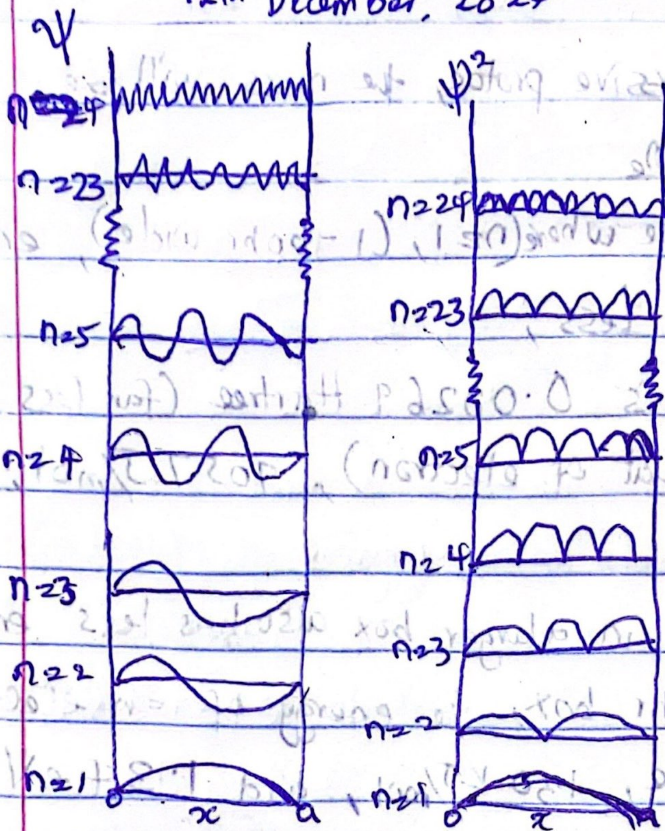
Fig 6. Particle in a box wave function!
