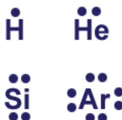
Figure 2- 8: Atoms in “dot notation”
