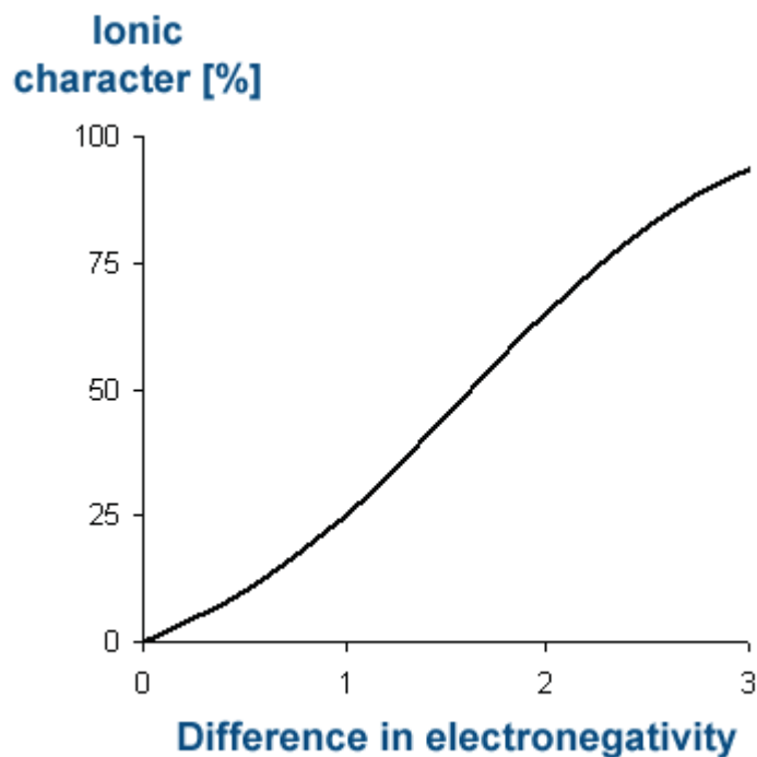
Figure 2- 24: Ionic character
