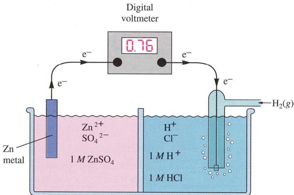
Figure 6- 2: Galvanic cell
