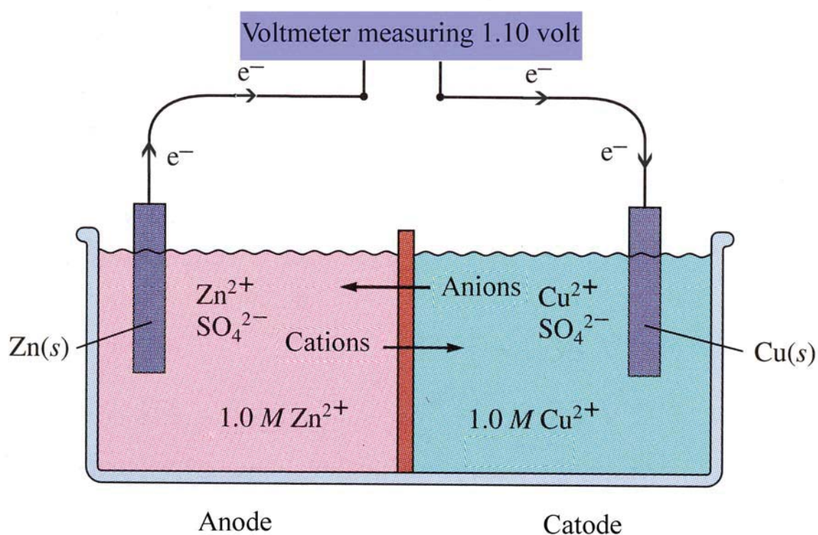
Figure 6- 12: Zinc/cobber galvanic cell
