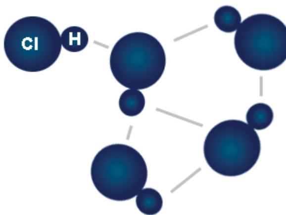
Figure 2- 2: Dipole-dipole forces among HCl molecules
