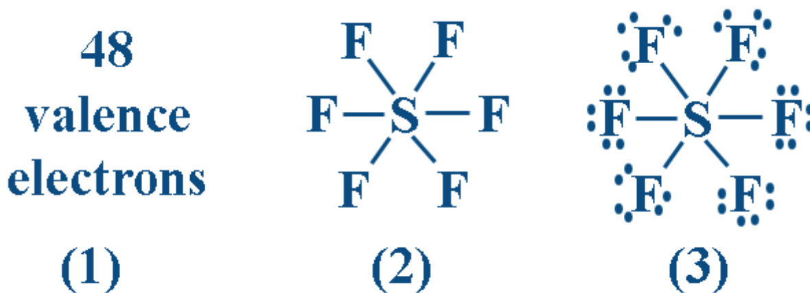
Figure 2- 11: Lewis structure for the sulphur hexafluoride molecule
