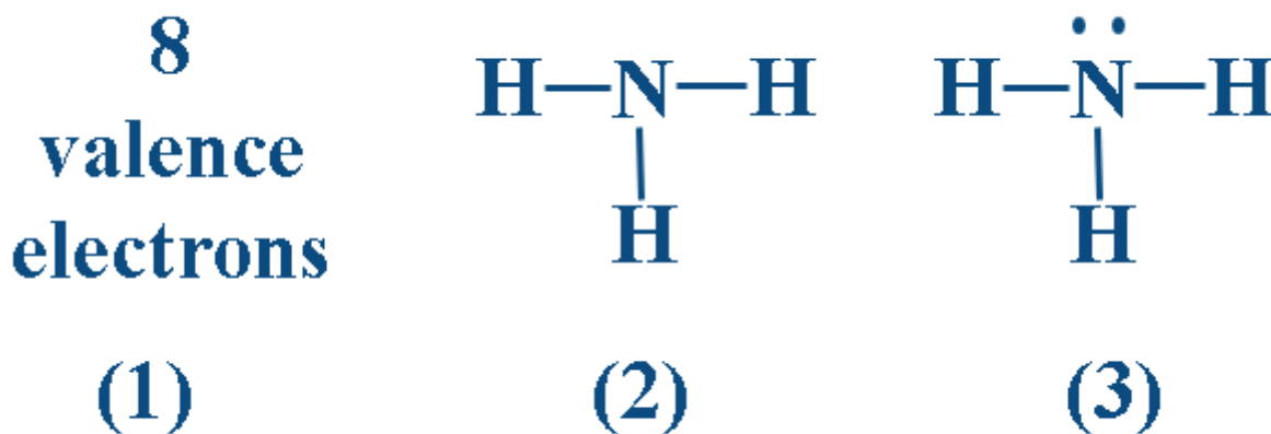
Figure 2- 9: Lewis structure for the ammonia molecule
