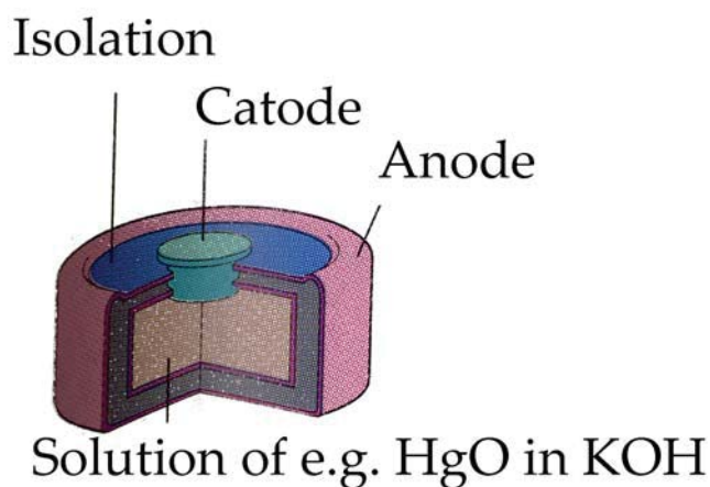
Figure 6- 8: Mercury battery Sketch of a basic mercury dry cell battery.
