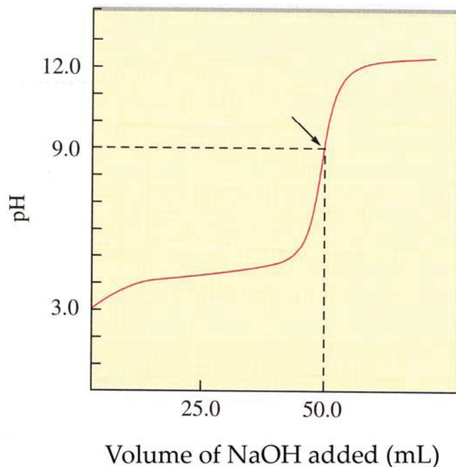
Figure 5- 2: Titration curve pH profile for a titration of 50.0 mL \text{CH}_3\text{COOH} with a 0.10 M NaOH solution.
