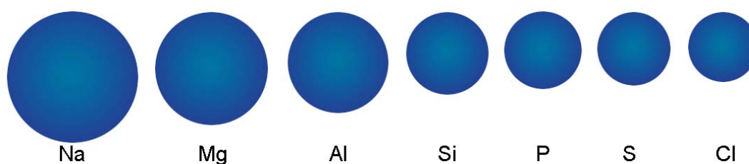
Figure 1- 9: Relative atomic radius for 3 rd period elements Relative atomic radius for the elements in the 3 rd period of the periodic table.
