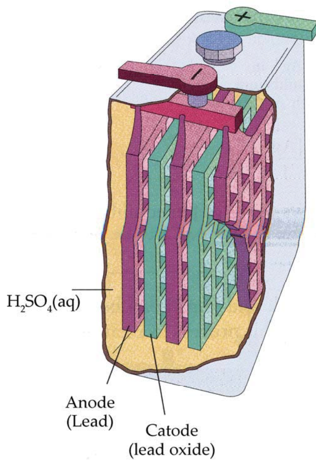
Figure 6- 6: The lead battery The set-up in a lead battery.
