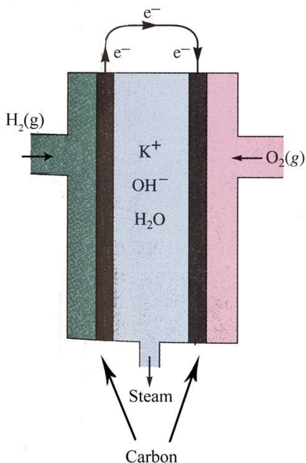
Figure 6- 9: Fuel cell
