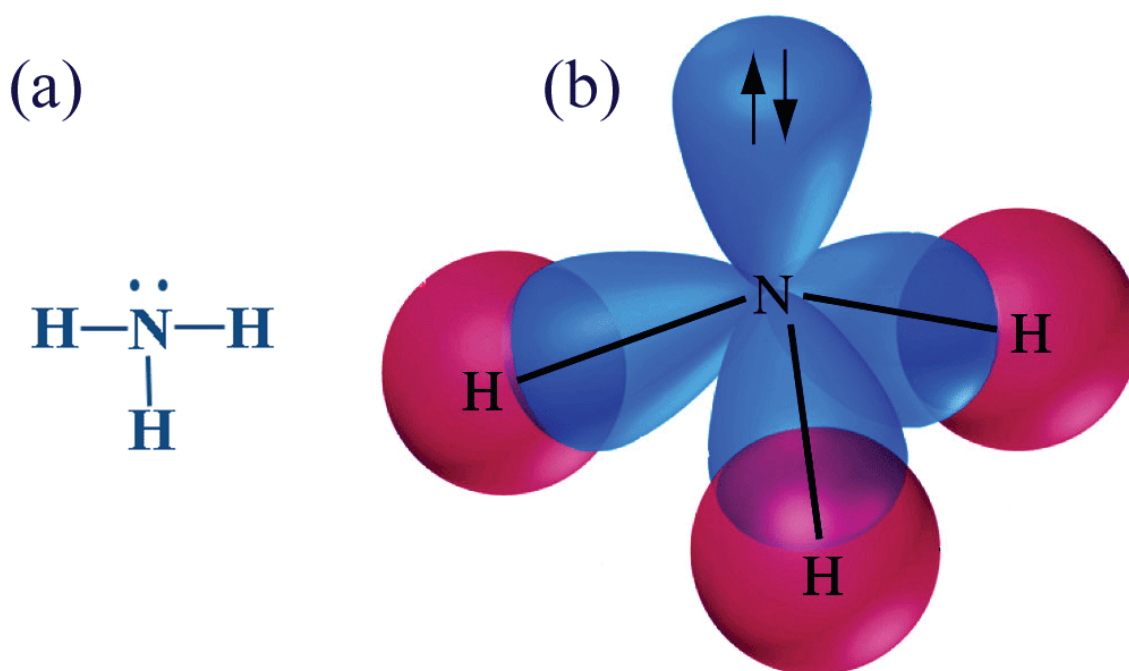
Figure 2- 16: sp 3 -hybridization in NH 3
